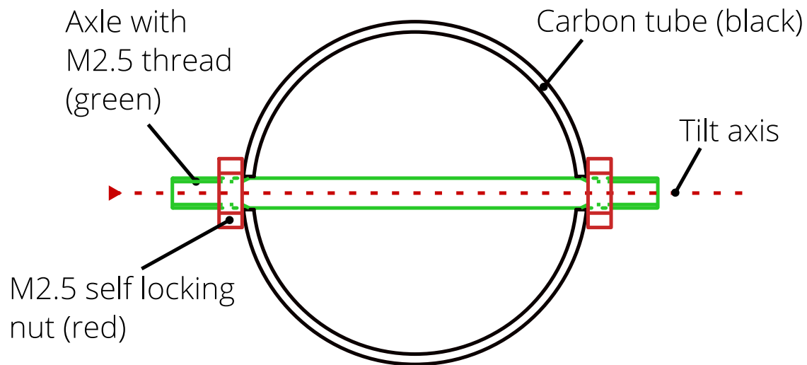
Figure 2 – Tilt mechanism, seen from the front
